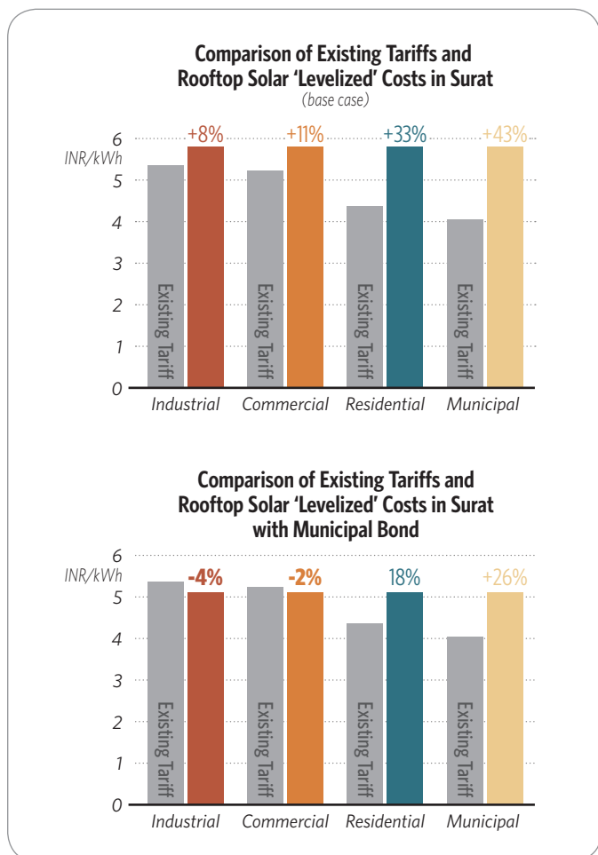
Figure 6: Comparison of existing electricity tariffs with rooftop solar LCOE with and without municipal bonds for Surat
