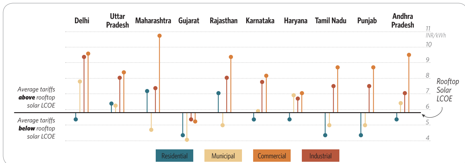
Figure 4: Average electricity tariffs for different states and market segments and rooftop solar LCOE
