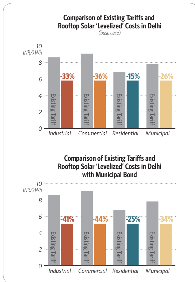
Figure 7: Comparison of existing electricity tariffs with rooftop solar LCOE with and without municipal bonds for New Delhi
